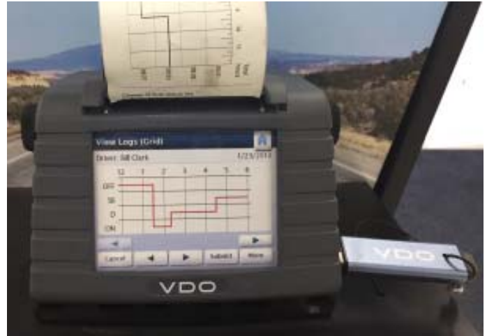
RoadLog recorder, printer and flash drive key
